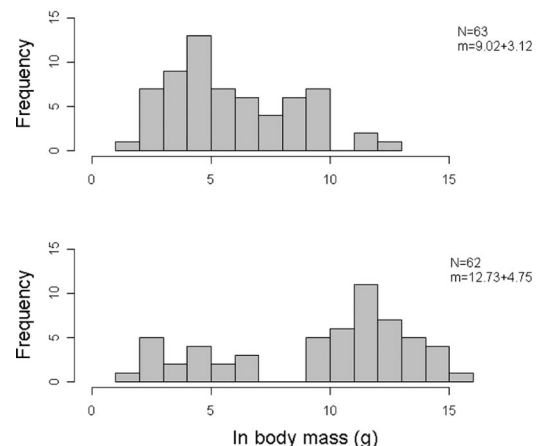
Fig. 3. Histograms of ln body mass of SLOH (Upper) and non-SLOH (Lower) genera. N , sample size; m , mean ln body mass (in grams). See Fig. S3 for an alternative plot of this figure.
